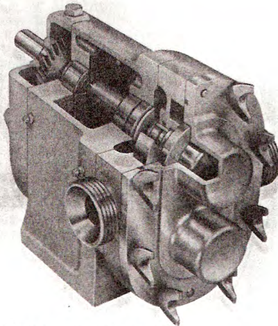
Metal Rotor/Single O-ring Design
